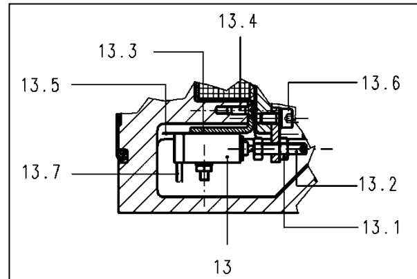
Fig. 21/1: Microswitch adjustment
