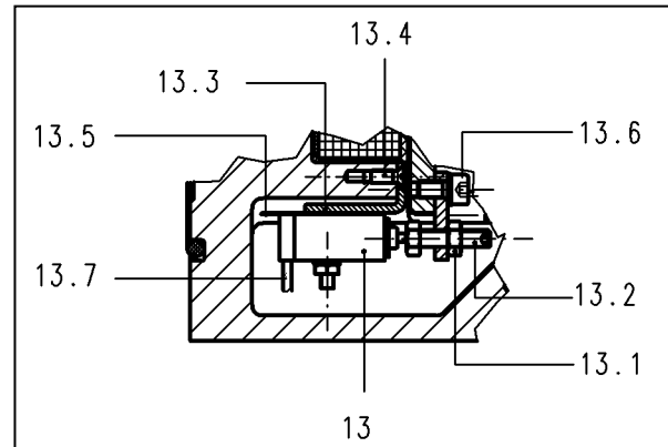
Fig. 24/1: Microswitch adjustment
